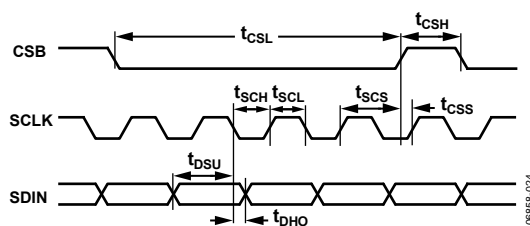
Figure 3. SPI Timing
