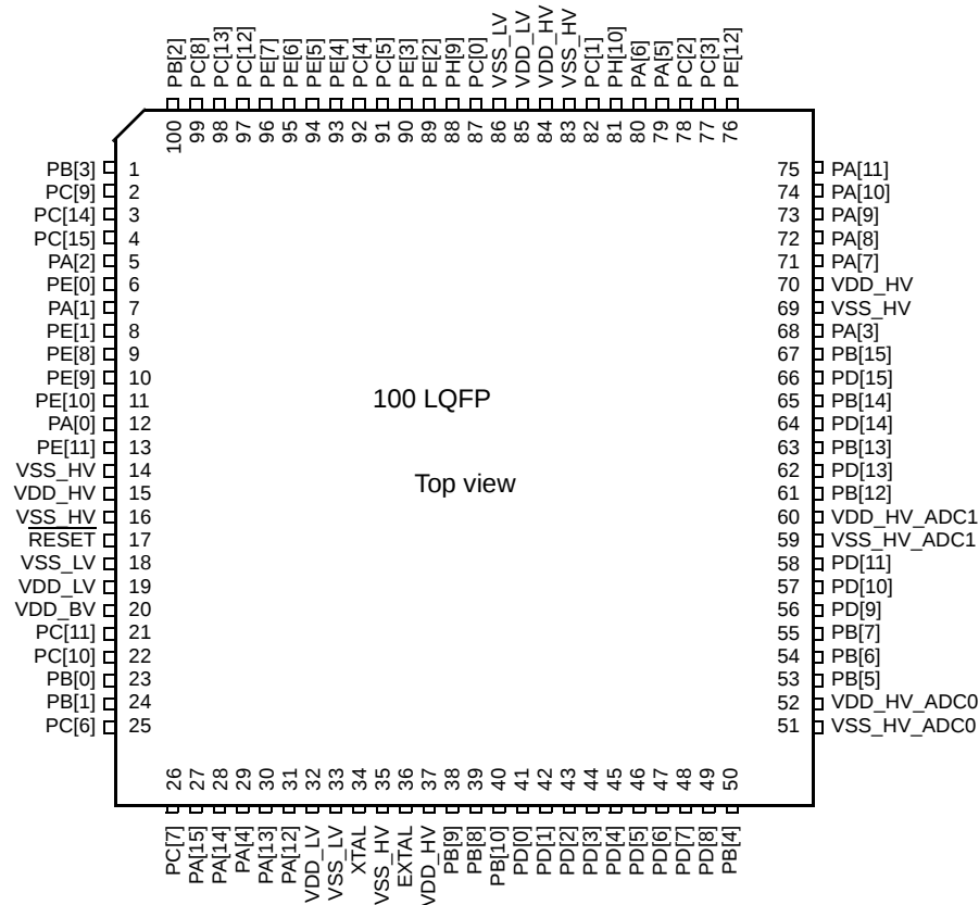
Figure 4. 100 LQFP pinout
