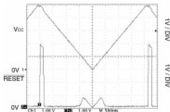
Fig. 8: SP705/707 RESET Output Voltage vs. Supply Voltage
