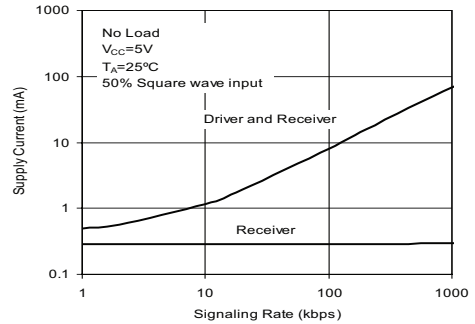
Supply Current vs Signaling Rate (SP3083E-SP3085E)
