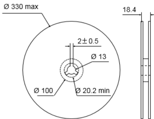
Figure 18. Reel dimensions (mm)
