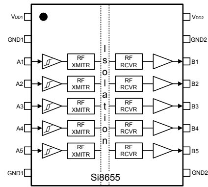
Figure 5.2. Si8655 Pinout
