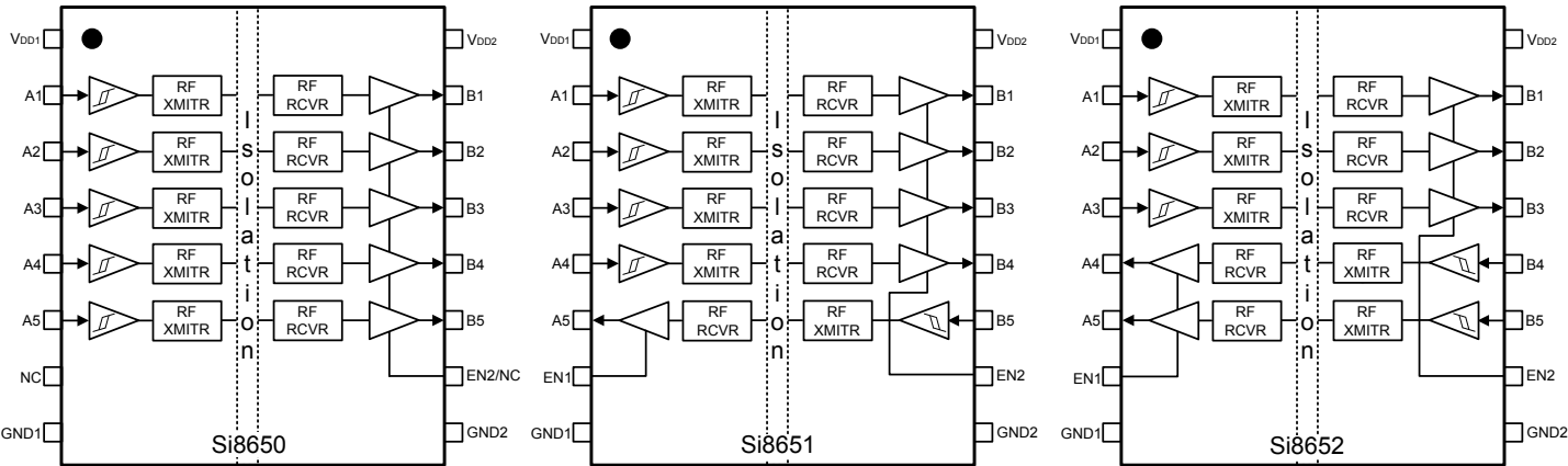
Figure 5.1. Si8650/51/52 Pinout
