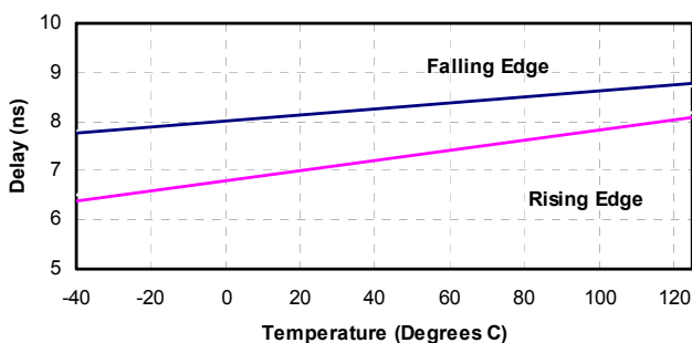
Figure 11. Propagation Delay vs. Temperature
