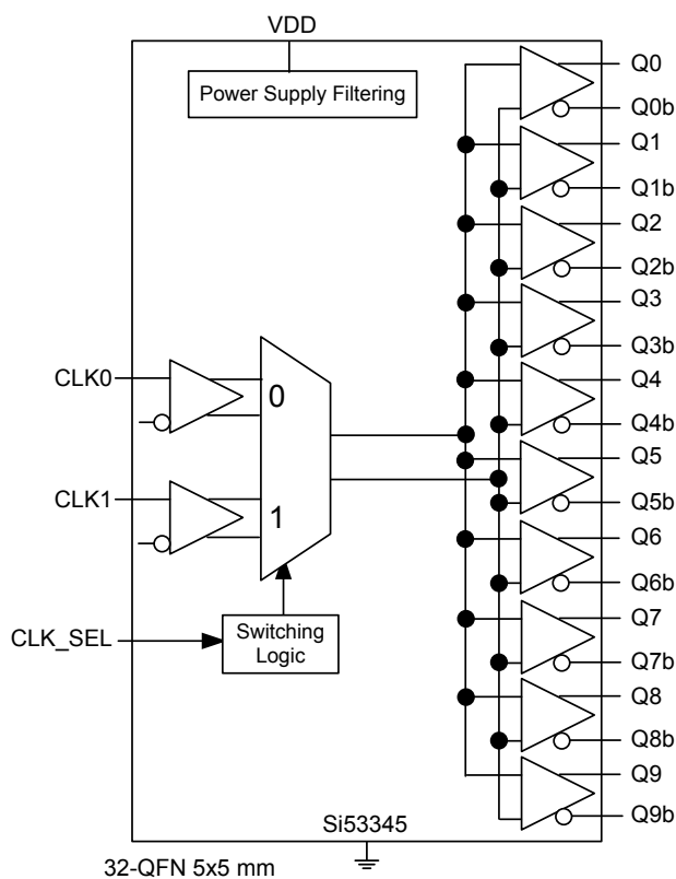
Figure 4.6. Si53345 Block Diagram
