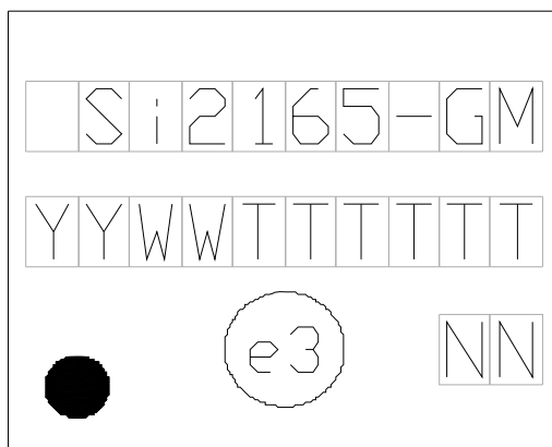
Figure 26. Top Mark
