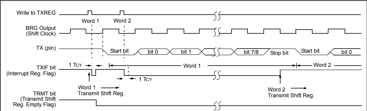
FIGURE 17-5: ASYNCHRONOUS TRANSMISSION (BACK TO BACK)
