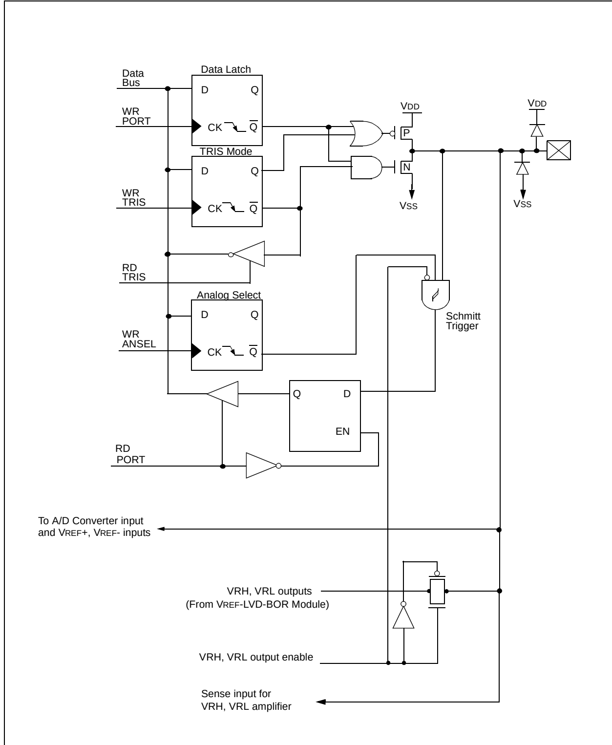
FIGURE 3-2: BLOCK DIAGRAM OF RA2/AN2/V REF- /VRL AND RA3/AN3/V REF+ /VRH
