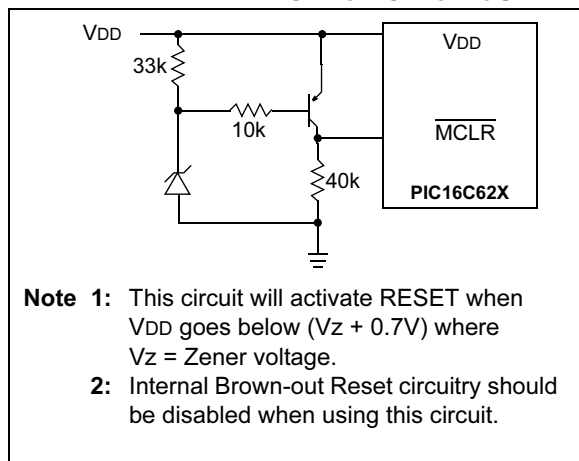
FIGURE 9-12: EXTERNAL BROWN-OUT PROTECTION CIRCUIT 1
