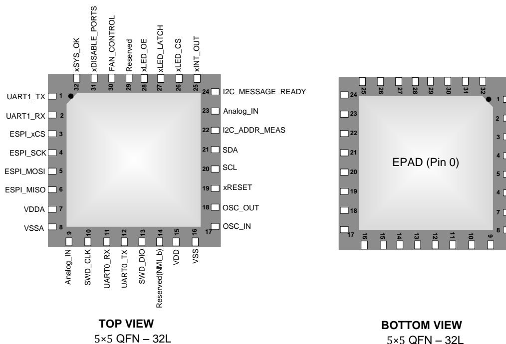
Figure 3: PD69200 Pinout
