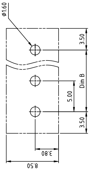
RECOMMENDED P.C.B LAYOUT TOP VIEW
