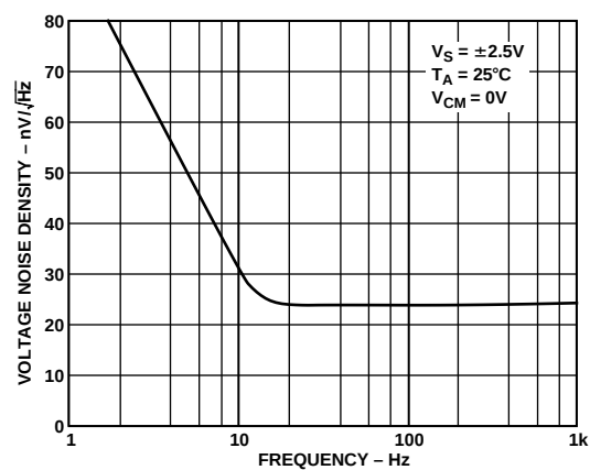
TPC 27. Voltage Noise Density vs. Frequency
