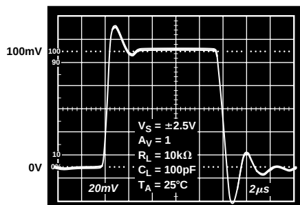
TPC 31. Small Signal Transient Response
