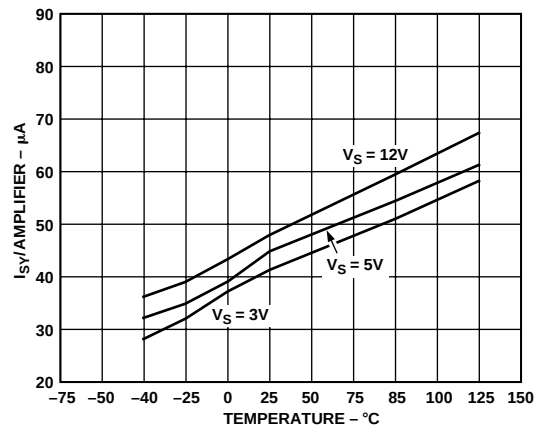
TPC 25. Supply Current/Amplifier vs. Temperature
