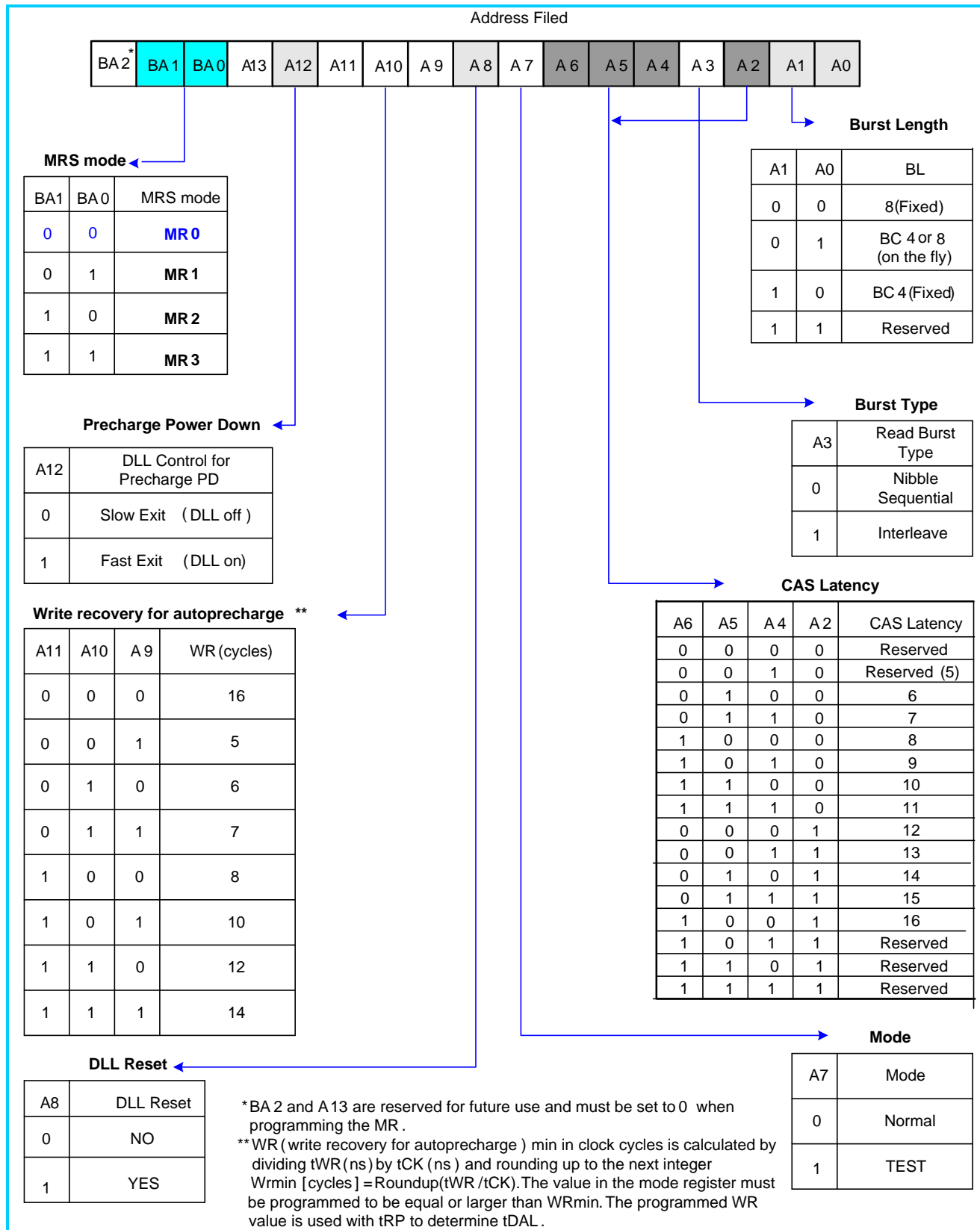
Fig. 8:MR0 Definition
