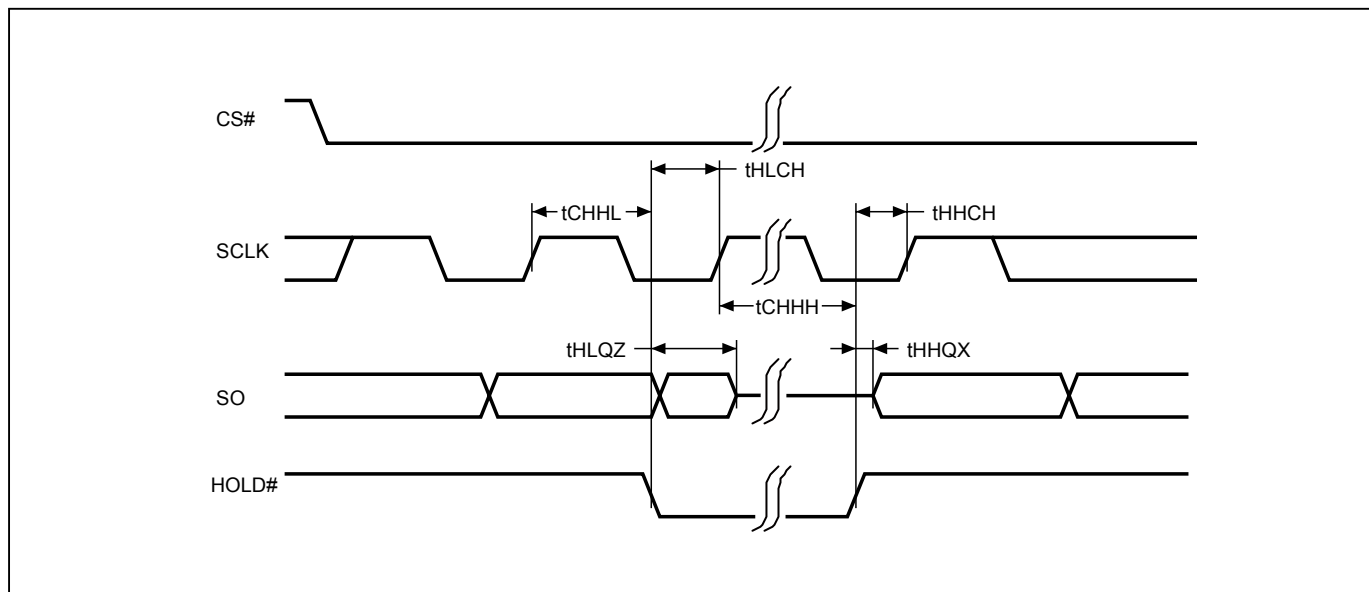
Figure 9. Hold Timing
