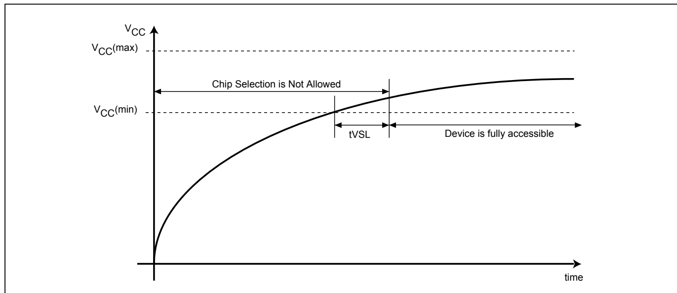
Figure 27. Power-up Timing
