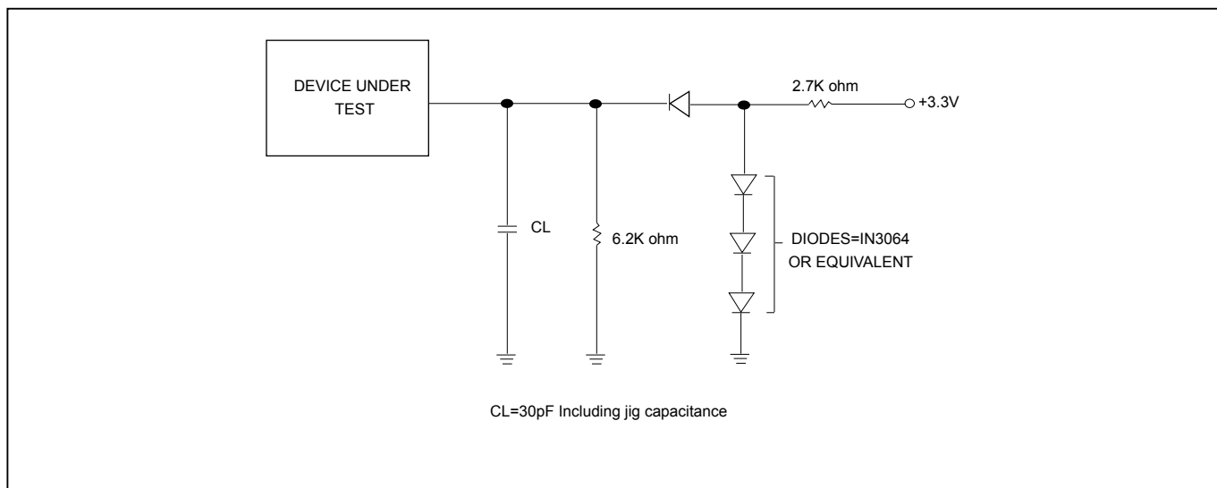
Figure 6. OUTPUT LOADING
