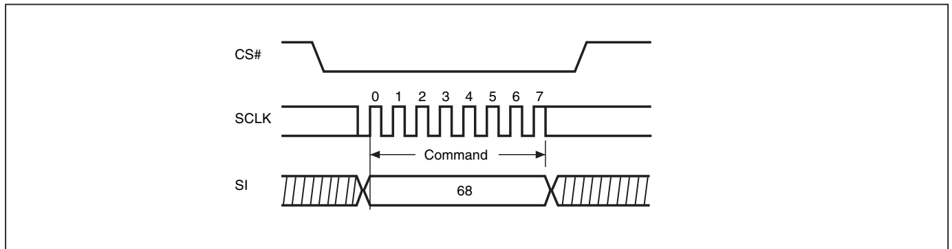
Figure 37. Write Protection Selection (WPSEL) Sequence (Command 68)
