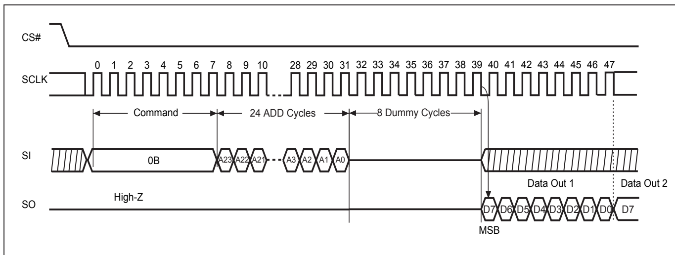
Figure 18. Read at Higher Speed (FAST_READ) Sequence (Command 0B)
