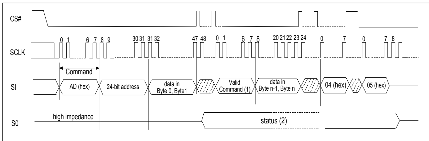
Figure 31. Continuously Program (CP) Mode Sequence with Hardware Detection (Command AD)
