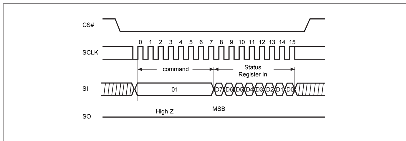
Figure 16. Write Status Register (WRSR) Sequence (Command 01)
