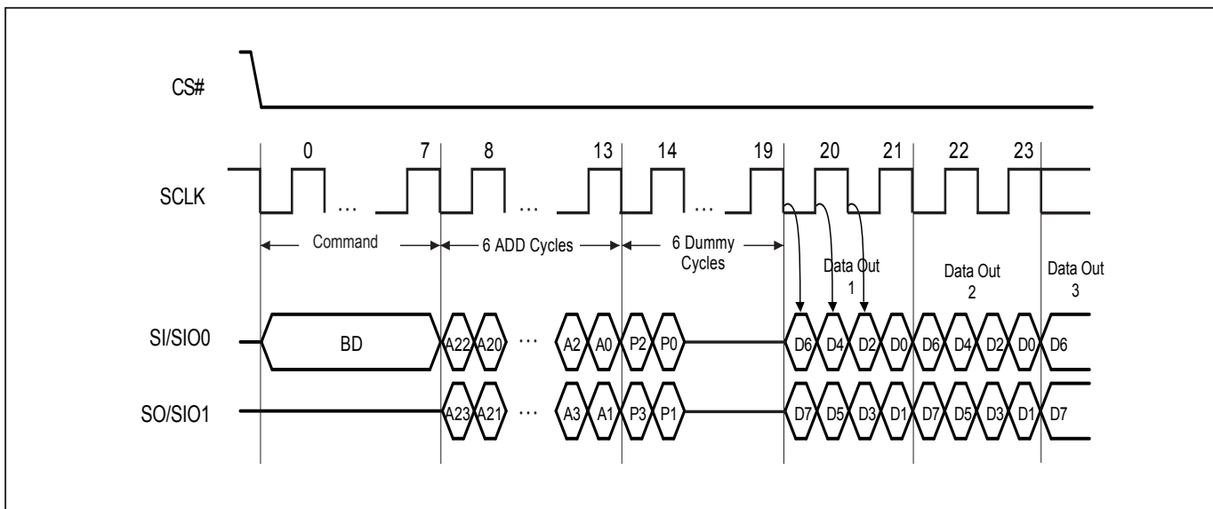
Figure 21. Fast Dual I/O DT Read (2DTRD) Sequence (Command BD)
