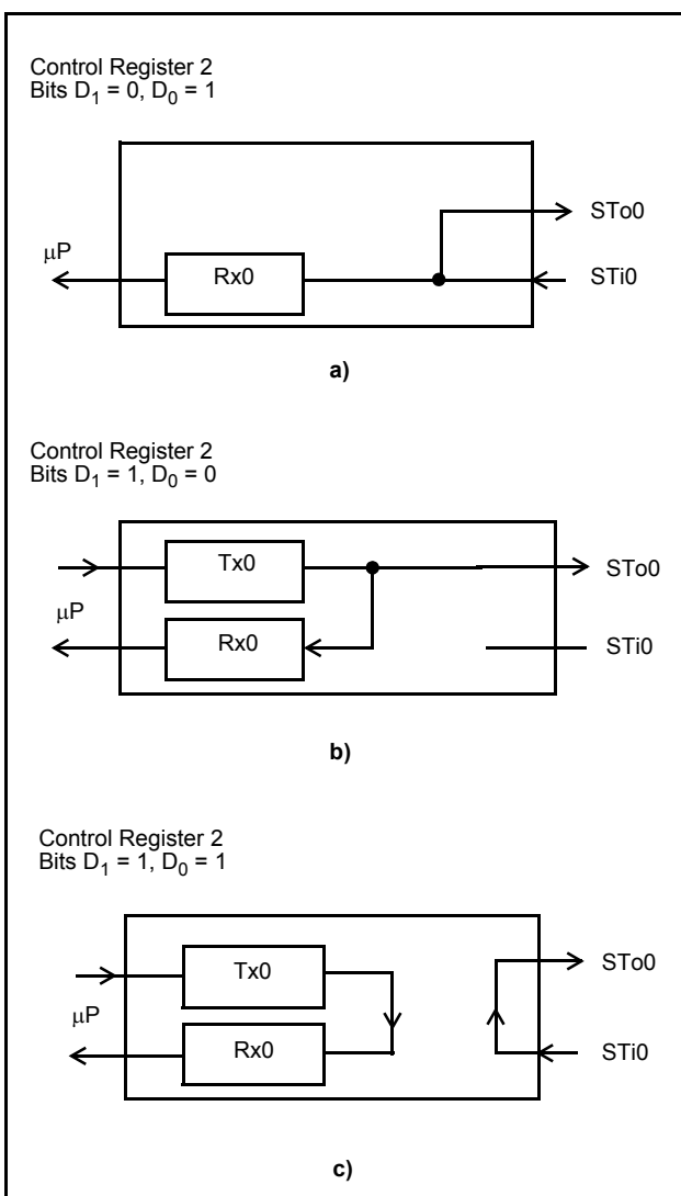
Figure 5 - Loopback Configurations
