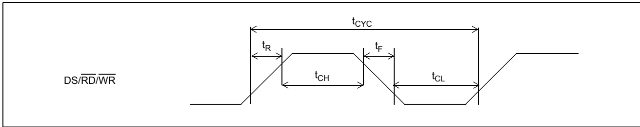
Figure 18 - \overline{\text{DS/RD/WR}} Clock Pulse
