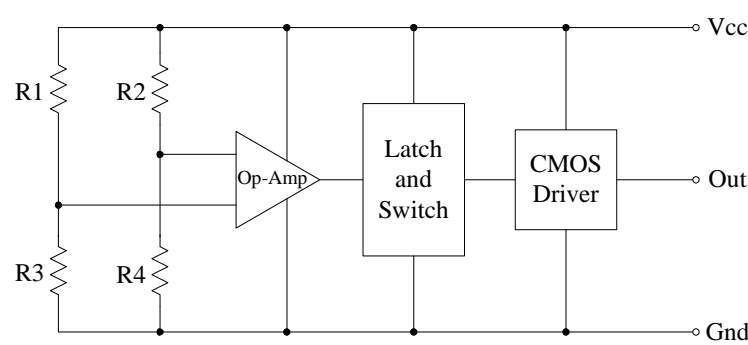
The intermittent switch circuit inside
