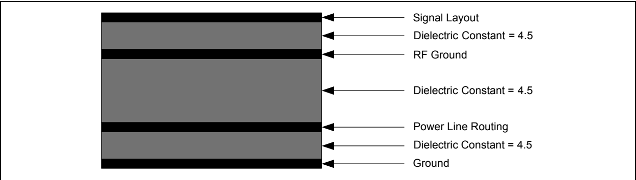
FIGURE 4-4: FOUR BASIC COPPER FR4 LAYERS
