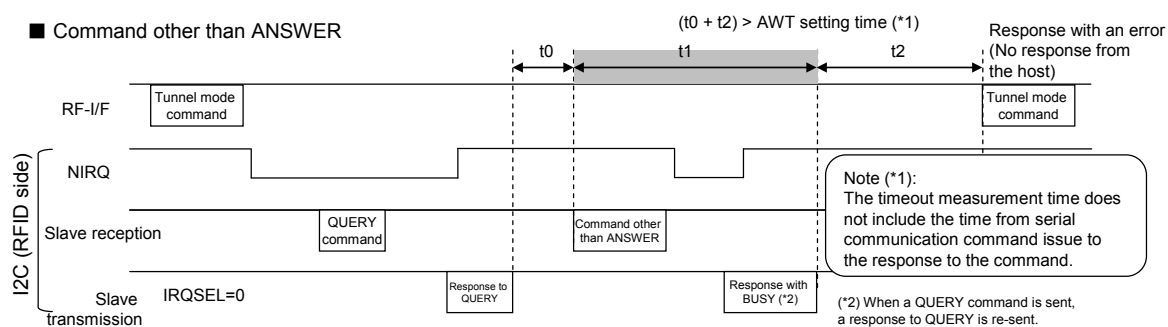
Figure 7-7 Timeout of Waiting for ANSWER Command (Command Other Than ANSWER)
