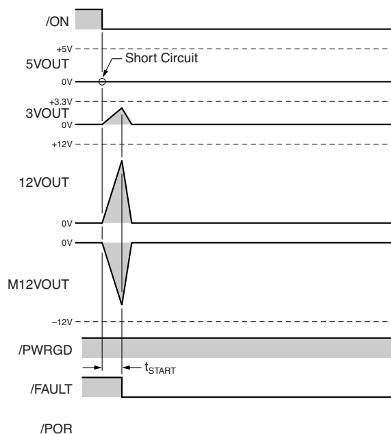
Figure 2. Controller Timing: Enable Into Short
