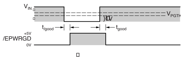
Figure 4. Early Power Good Response Time
