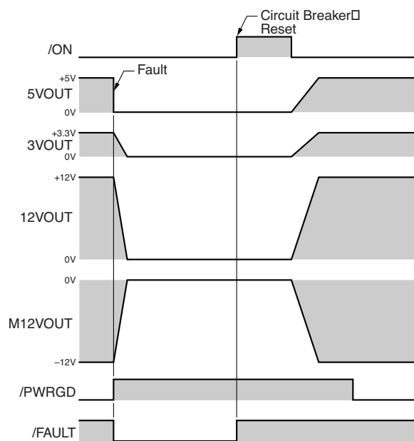
Figure 3. Controller Timing: Short on 5V
