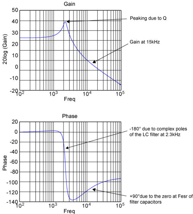
Figure 12. Modulator Transfer Function
