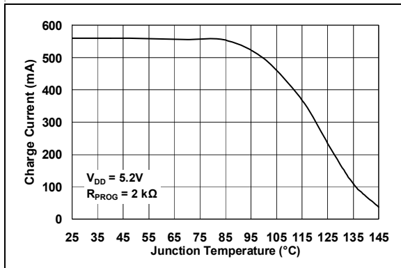
FIGURE 5-1: Thermal Regulation.
