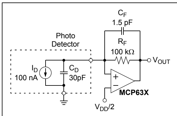
FIGURE 4-11: Transimpedance Amplifier for an Optical Detector.
