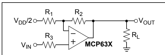
FIGURE 4-10: Power Driver.
