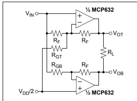
FIGURE 4-12: H-Bridge Driver.
