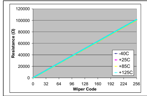
FIGURE 2-57: 100 kΩ – R_{WB} ( \Omega ) vs. Wiper Setting and Ambient Temperature ( V_{DD} = 5.5\text{V} , I_W = 45\text{ }\mu\text{A} ).
