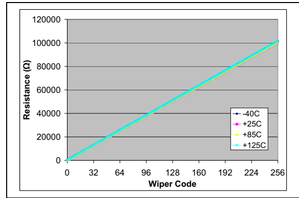
FIGURE 2-58: 100 kΩ – R_{WB} ( \Omega ) vs. Wiper Setting and Ambient Temperature ( V_{DD} = 3.0\text{V} , I_W = 24\text{ }\mu\text{A} ).
