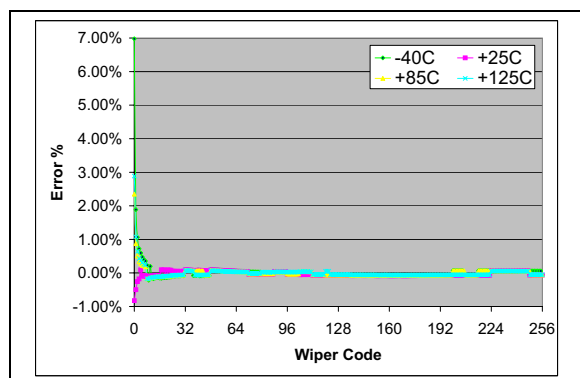
FIGURE 2-44: 50 kΩ – Worst Case R_{BW} from Average R_{BW} ( R_{BW0} - R_{BW3} ) Error (%) vs. Wiper Setting and Temperature ( V_{DD} = 5.5\text{V} , I_W = 90\text{ }\mu\text{A} ).
